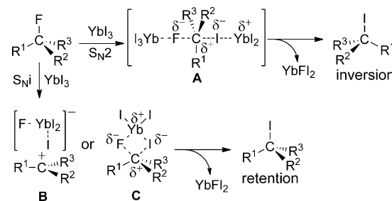
Scheme 4. Mechanistic proposal for the F/I substitution.
