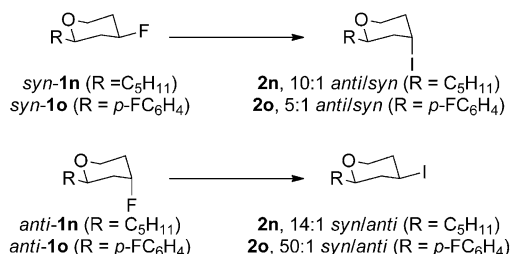
Scheme 3. Stereochemical analysis of tetrahydropuran derivatives 1n and 1o . Reaction conditions: YbI_3 (0.0484 mmol, 2.42 mm), \text{CH}_2\text{Cl}_2 (2 mL), substrate (0.044 mmol, 2.2 mm).
